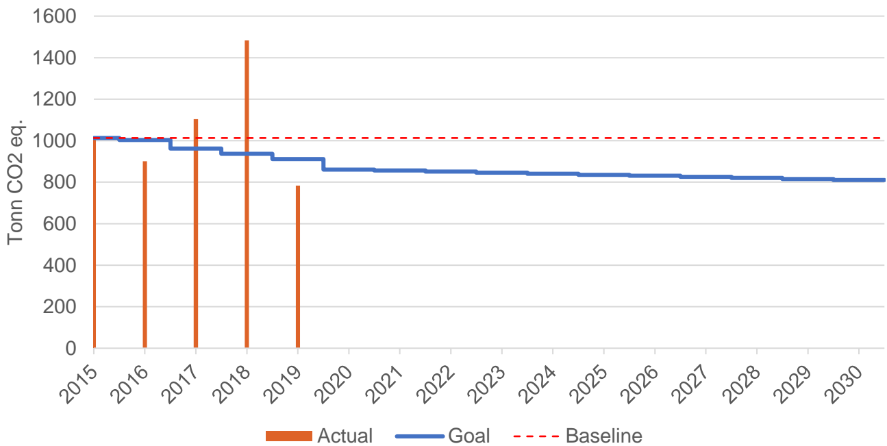
Emissions from Construction and Maintenance
